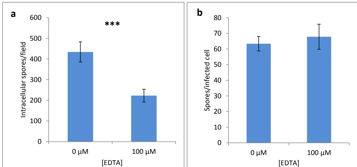
Figure 3.2: EDTA-mediated infection response of Anncaliia algerae in goldfish skin cells (GFSk-S1) eight days post-inoculation. Intracellular spores per field (a) were significantly reduced by EDTA treatment (p=3.38*10 -10 ). b) The average number of spores per infected cell was not significantly affected (p=0.35). Counts determined by random micrographs (n=5 micrographs/well for 8 replicate wells/treatment) pooled from eight replicate treatments. Error bars indicate 95% CI.
