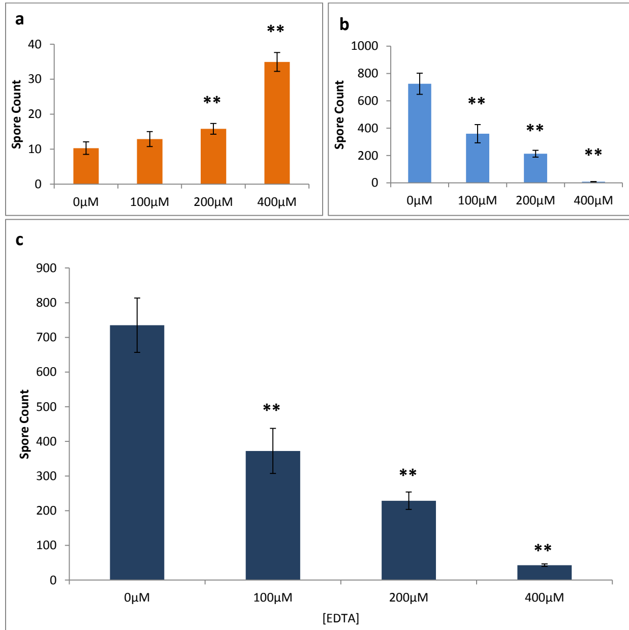
Figure 3.3: Haemocytometer counts of spores recovered from infected flasks eight days post-inoculation (n=5 replicates/treatment). a) Increased EDTA concentrations resulted in larger numbers of free-floating spores recovered from media ( p = 1.741 \times 10^{-9} ), (b) reduced numbers of infecting spores recovered by Percoll® centrifugation ( p = 1.035 \times 10^{-8} ), and (c) reduced total spore numbers ( p = 2.516 \times 10^{-8} ; chart c). Error bars indicate 95% CI.
